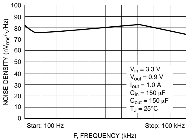
Figure 12. Noise Density vs. Frequency
