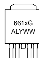
DPAK-5 CENTER LEAD CROP CASE 175AA
